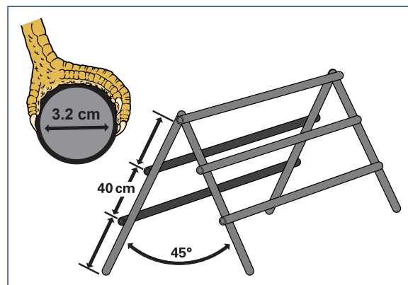
A-frame perch design
